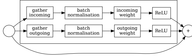
Fig. 2. Residual block used in the network. Note disjoint parameters for incoming and outgoing edges, both linear and normalisation layers.
