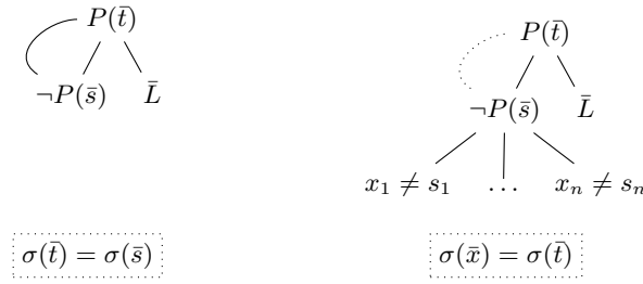
Fig. 1. Adding \neg P(\bar{s}) \vee \bar{L} to a tableau where P(\bar{t}) is the current goal. The left tableau shows conventional “strict” extension, the right LPCT “lazy” extension.
