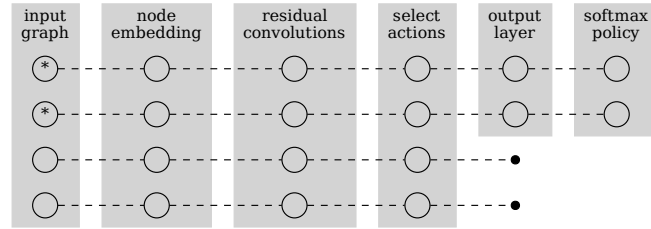
Fig. 3. Network diagram. As there is no pooling of any kind, data is processed at the node level until action nodes marked (*) are projected out.
